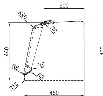
蓋切欠き部概略図(FREE)
